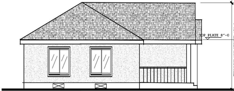
LEFT ELEVATION
